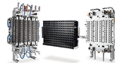
72腔瓶胚模具 72 Cavity Preform Mould
