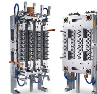
32腔瓶胚模具 32 Cavity Preform Mould
